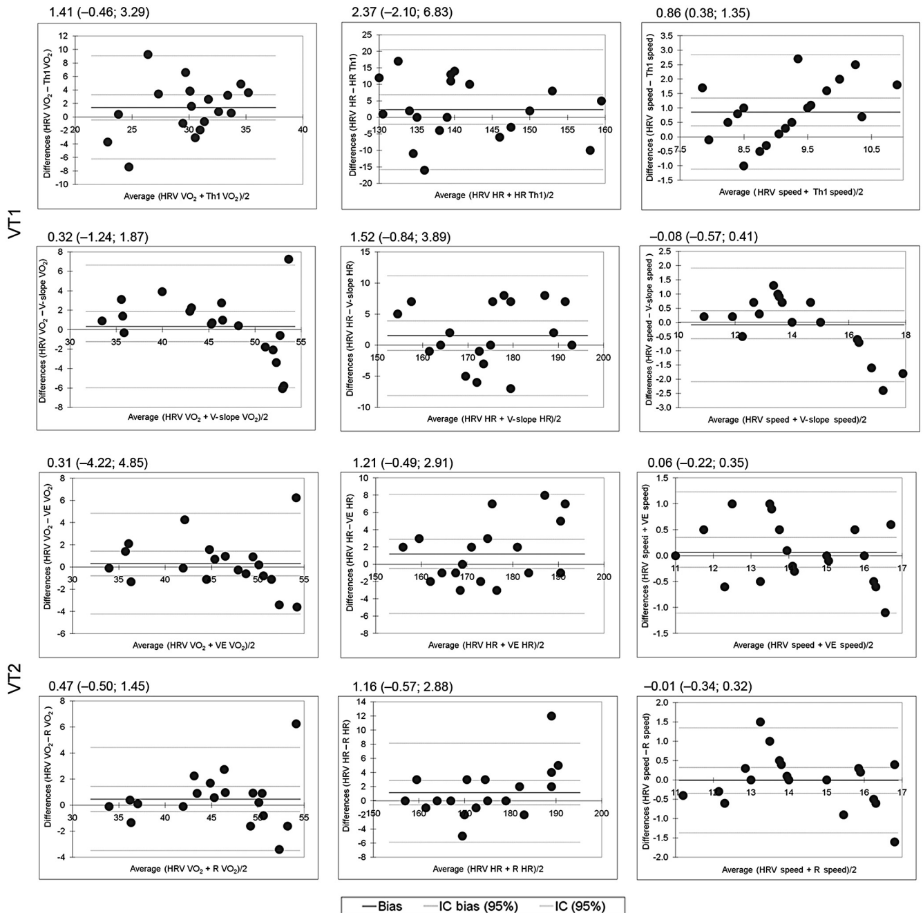
Fig. 1. Bland-Altman plots representing the central line and 95% limits of agreement between VT parameters, as assessed from HRV and from the gas analysis. HR = heart rate; HRV = heart rate variability; IC = interval of confidence; R = gas exchange ratio; Th = threshold; Th1 = aerobic threshold; VE = ventilatory equivalent; VO 2 = oxygen consumption; V-slope = slope trends; VT = ventilator threshold.
