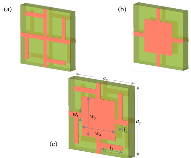
Fig. 1. (a) CCMM [3], (b) estructura fishnet modificada y (c) FCMM propuesta. Dimensiones: l_1 = 3.7 mm, l_2 = 0.95 mm, w_t = 0.7 mm, w_x = w_y = 5.6 mm, a_x = a_y = 10 mm.
