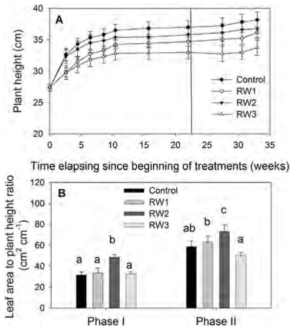
Fig. 2. Influence of the different irrigation treatments on plant height evolution throughout the experiment (A) and on leaf area to plant height ratio at the end of Phase I and Phase II (B) in M. communis plants. Vertical line indicates irrigation change between the end of the Phase II and the beginning of Phase II. Data represent the mean \pm SE from at least 6 plants. Different letters indicate significant differences ( P < 0.05 ) according to Duncan's test ( p < 0.05 ).
