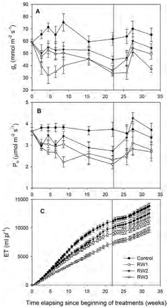
Fig. 4. Influence of the different irrigation treatments on stomatal conductance ( g_s ; A), net photosynthetic rate ( P_n ; B) and accumulated evapotranspiration (ET; C) in M. communis plants during the experiment. Vertical lines indicate irrigation change between the end of the Phase II and the beginning of Phase II.
