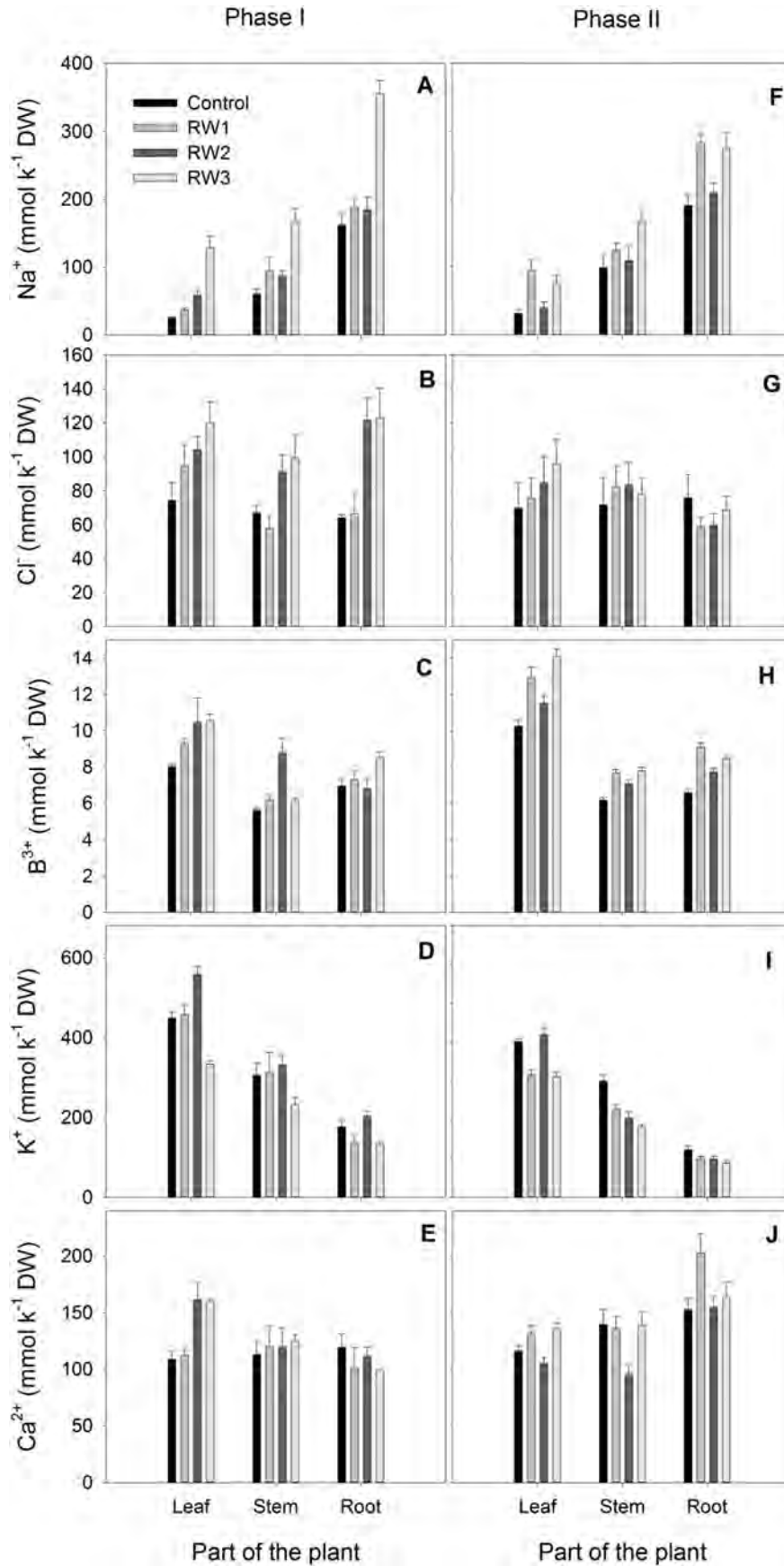
Fig. 6. Concentrations of \text{Na}^+ , \text{Cl}^- , \text{B}^{3+} , \text{K}^+ and \text{Ca}^{2+} in M. communis plants at the end of Phase I (A–E) and Phase II (F–J). Data represent the mean \pm SE from at least 6 plants. Different letters indicate significant differences ( P < 0.05 ) according to Duncan's test ( p < 0.05 ).
