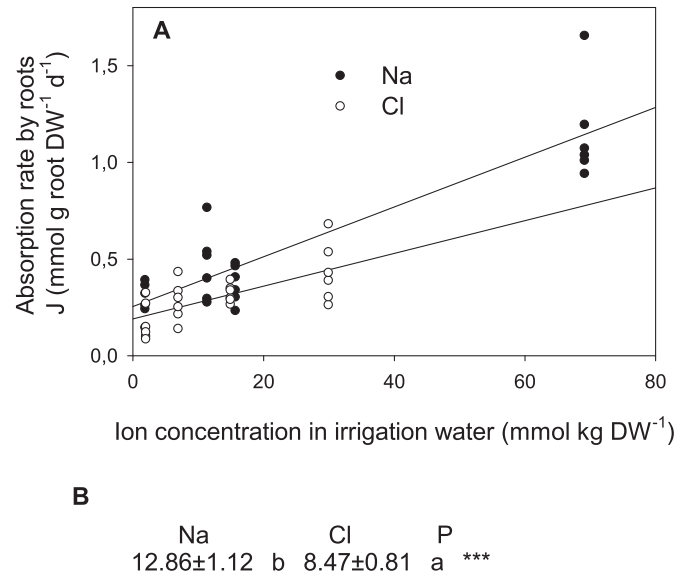
Fig. 5. (A) Absorption rate by roots (J) in M. communis plants at the end of Phase I. (B) The slopes of linear regressions between Na or Cl concentration in the irrigation water and absorption rate by roots (J) in M. communis plants at the end of Phase I are shown in the bottom part of the figure.
