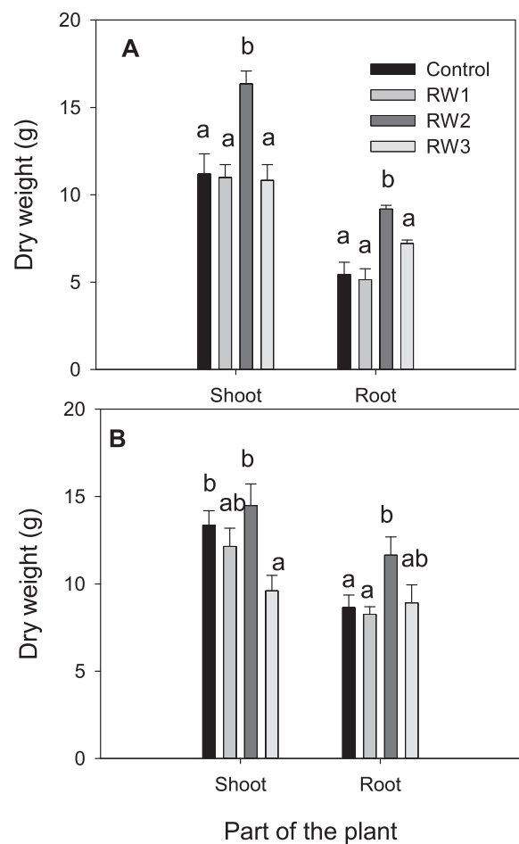
Fig. 1. Influence of the different irrigation treatments on biomass accumulation in M. communis plants at the end of Phase I (A) and Phase II (B). Data represent the mean \pm SE from at least 6 plants. Different letters indicate significant differences ( P < 0.05 ) according to Duncan's test ( p < 0.05 ).
