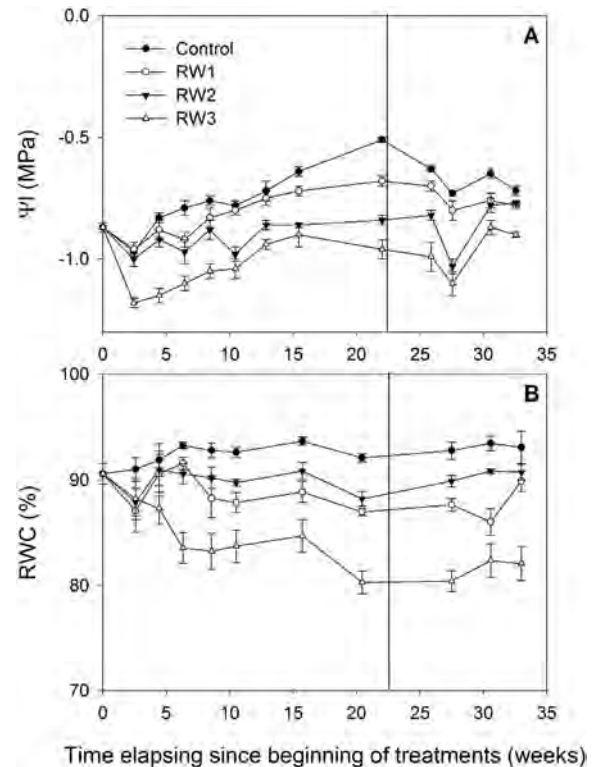
Fig. 3. Influence of the different irrigation treatments on leaf water potential ( \psi_1 ; A) and leaf relative water content (RWC; B) in M. communis plants during the experiment. Vertical lines indicate irrigation change between the end of the Phase I and the beginning of Phase II.
