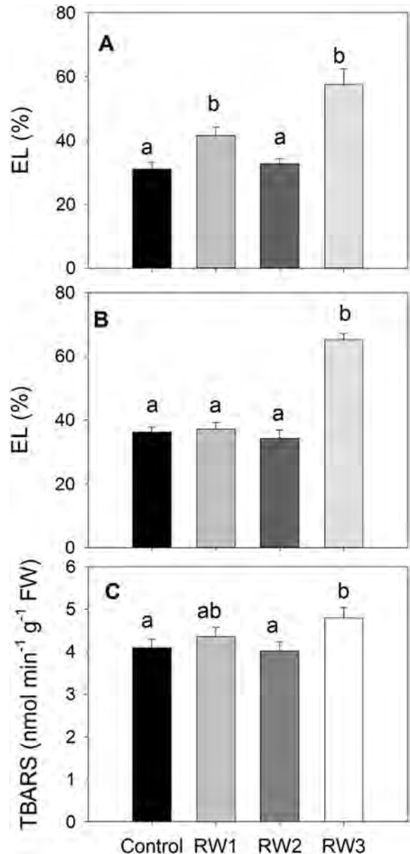
Fig. 7. Influence of the different irrigation treatments on oxidative stress parameters in leaves from Myrtus communis plants. Electrolyte leakage (EL) was analyzed at the end of Phase I (A) and Phase II (B) of the experiment, whereas lipid peroxidation (TBARS) was analyzed only after the stress period (C). Data represent the mean ± SE from at least 6 plants. Different letters indicate significant differences ( P < 0.05 ) according to Duncan's test ( p < 0.05 ).
