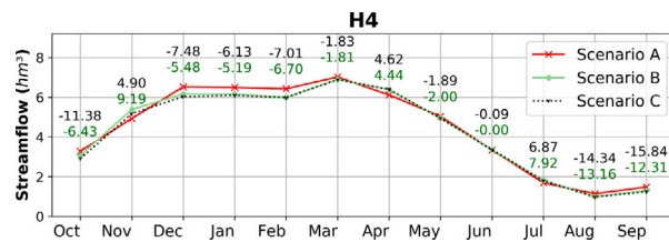
Fig. 5. Monthly streamflow mean simulations under scenarios A, B and C with the changes expressed in percentages for scenario A-B (green) and for scenario A-C (black). (For interpretation of the references to colour in this figure legend, the reader is referred to the web version of this article.)
