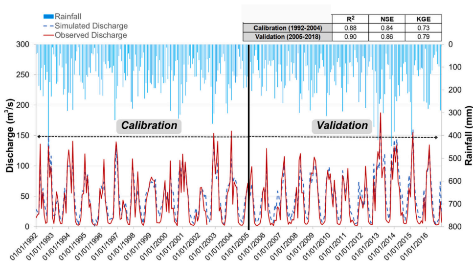
Fig. 3. Monthly calibration and validation time-series and statistical values.
